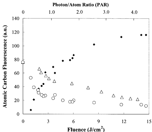
Fig. 2. Two-laser fragmentation by 193 nm photons of soot particles in air. The atomic carbon fluorescence produced by the first laser is shown as filled diamonds, and the fluorescence produced by the second pulse is shown as open circles (1 \mu s) and open triangles (100 ns). The fluence of the first pulse varies from 0 to 14.7 \text{J}/\text{cm}^2 , while the second pulse is constant at 13 \text{J}/\text{cm}^2 . These data are 100-shot averages taken at a laser repetition rate of 10 Hz.
