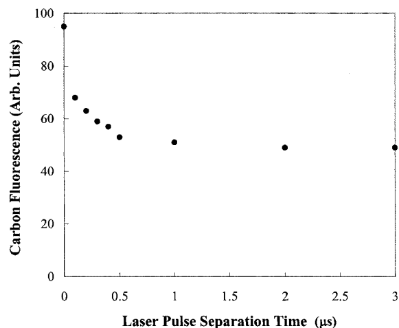
Fig. 3. Carbon fluorescence from the second laser pulse as a function of pulse separation time from 0 to 3 \mu s. The decrease in signal between laser pulses is likely due to oxidation of atomic carbon, carbon molecules, and soot particles remaining after the first laser pulse. The signal remains constant from 1 to 10 \mu s.
