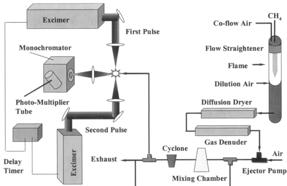
Fig. 1. Experimental apparatus.
