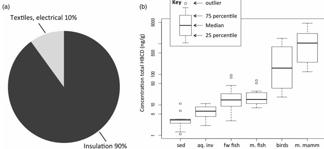
Figure 5 Hexabromocyclododecane (HBCD) usage and bioaccumulation. (A) The primary use of HBCD is in polystyrene building insulation. (B) HBCD in the food chain. Species at the top of the food chain have the highest levels of HBCD. The graph shows the concentration of HBCD in sediments (sed, ng/g dry weight) and biological samples (ng/g lipid weight). aq. inv. = aquatic invertebrates; fw fish = freshwater fish; m. fish = marine fish; and m. mamm = dolphins, porpoises. Source: Graphs created from data in Covaci et al. (2006)
